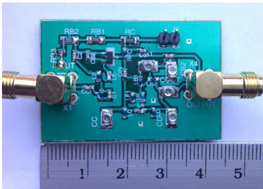
Gambar 8. Hasil Fabrikasi rangkaian co-design dual band LNA dan BPF
